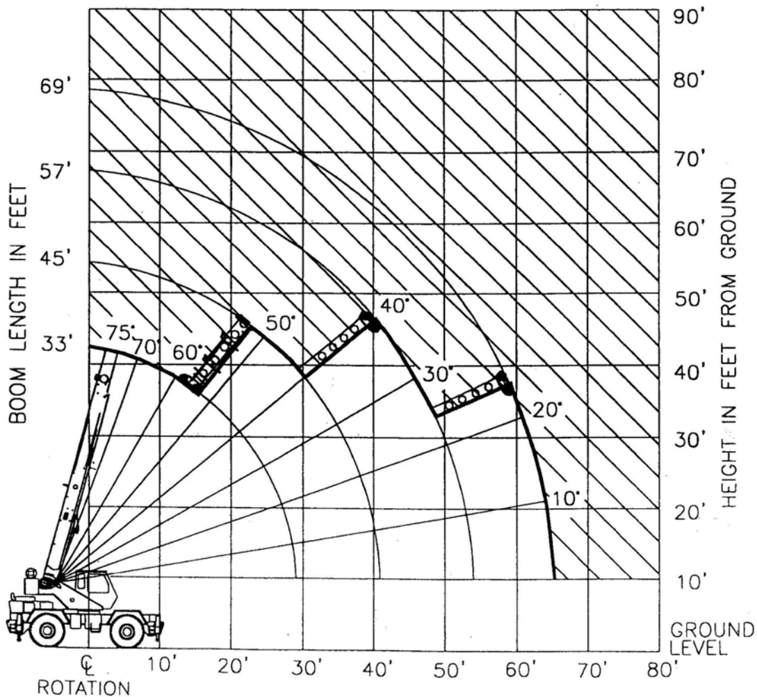
BOOM DEFLECTIONS NOT SHOWN
